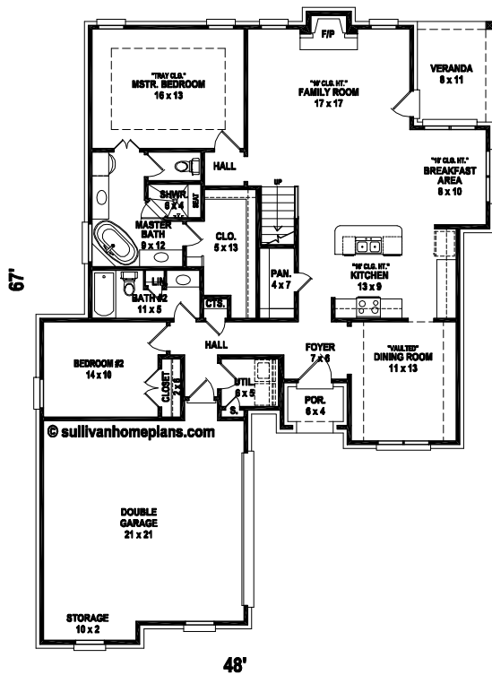
FIRST LEVEL FLOOR PLAN
