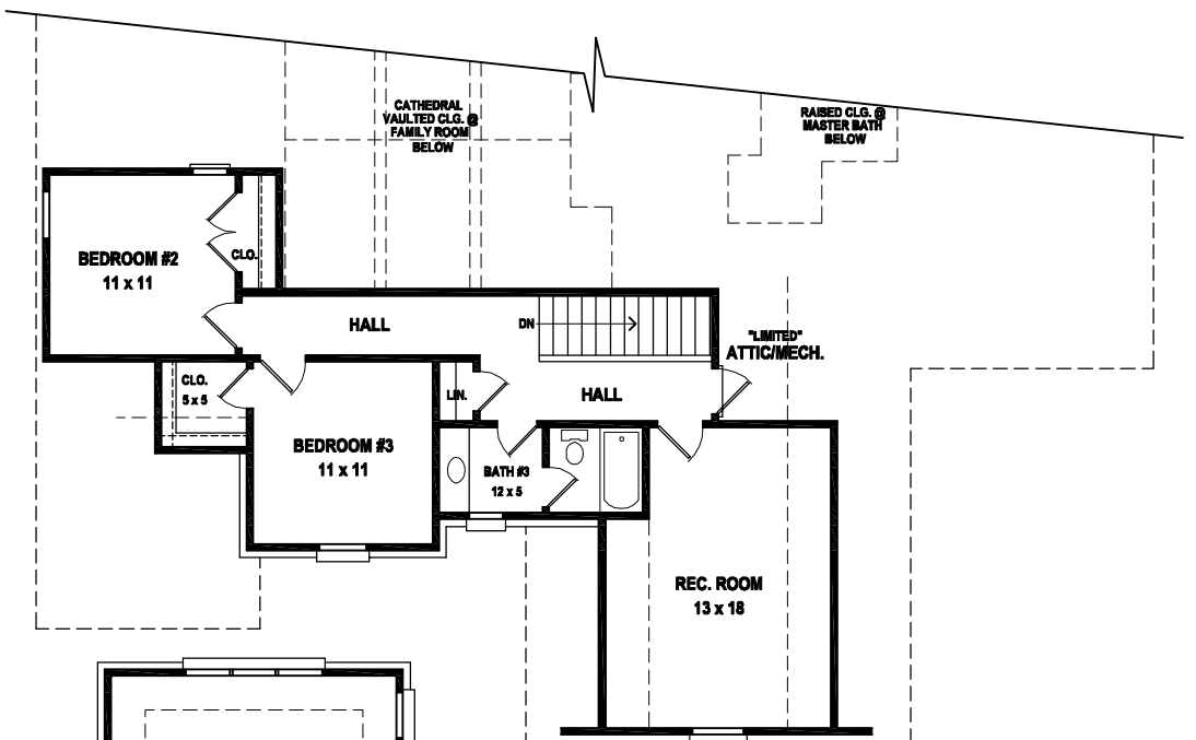
SECOND LEVEL FLOOR PLAN
