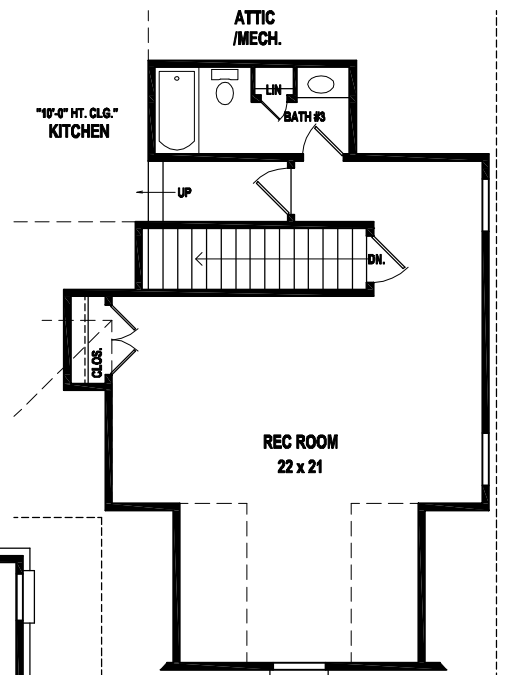
SECOND LEVEL FLOOR PLAN
